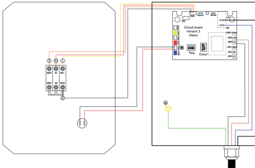
Secondary control box internal wiring
