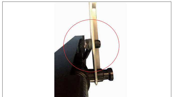
Step 20: Secure the Octagon drum lid to the cyclone funnel using hex bolts (8) 8 mm*19 mm, flat washers (16) 8 mm*OD18*2T and hex nuts (8) 8 mm. Make sure to first attach all the bolts on before tightening the bolts.
